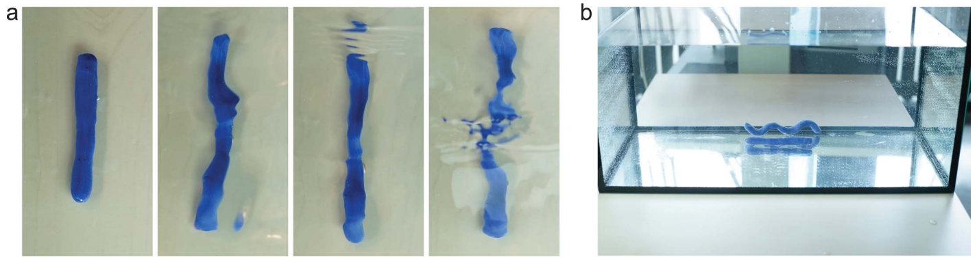
Figure 1. Refraction of light. (a) A piece of blue modeling clay is photographed under water, when the water is still (first image) and when it is wavy (remaining three images). Photographs show shape distortions and phase breaks due to the ripples on the water, making it impossible to recover the veridical shape of the modeling clay. (b) Photographing set-up viewed from the side reveals two different shapes of modeling clay inside a full water tank.
