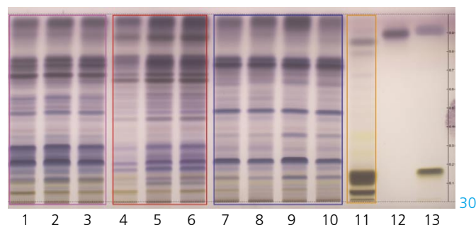
Differentiation of Hoodia species and prickly pear cactus: Tracks 1–3 Hoodia gordonii , 4–6 Hoodia currorii , 7–10 Hoodia parviflora , 11 prickly pear cactus ( Opuntia ficus indica ), 12 P57, 13 fructose (bottom), \beta -sitosterol (top).
