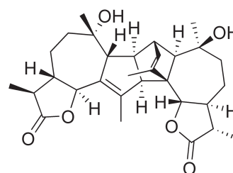
▲ Structure formula of absinthin
