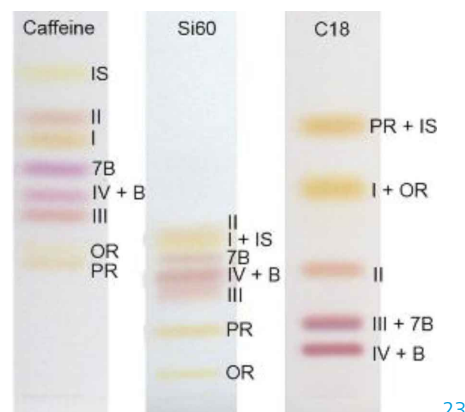
Separation of 8 azo dyes on caffeine-impregnated HPTLC plates NANO-SIL-PAH, HPTLC plates silica gel 60, and HPTLC plates RP 18 following [3]
