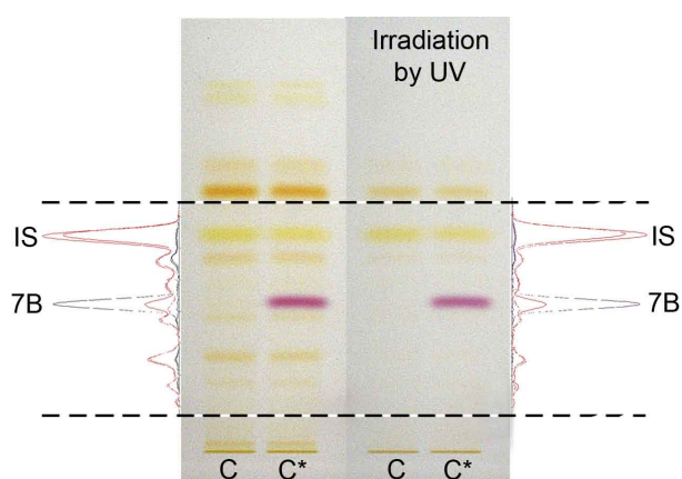
Effect of UV irradiation on the matrix background of the chromatogram for a native (C) and spiked (C*, Sudan Red 7B, 500 mg/kg) chili powder extract
