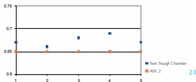
▲ R_F -values ( n = 15 ) of dimetridazole averaged across the plate (values from 5 plates), saturated 20 min with filter paper plus pre-conditioning 10 min. Relative standard deviation of the R_F -averages ( n = 5 ) now 1.6 % for the TTC and 0 % for the ADC 2.
