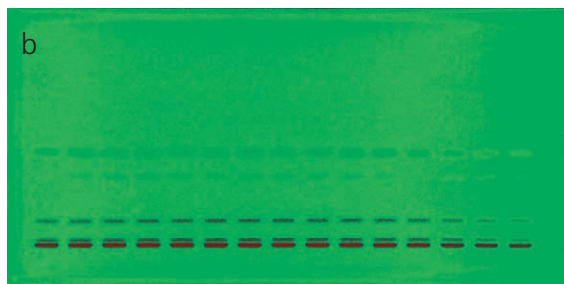
▲ Separation of a sulfonamide mixture in the saturated chamber (20 min, filter paper) with 10 min pre-conditioning of the layer; Twin Trough Chamber (a) and ADC 2 (b). Images under UV 254 nm.
