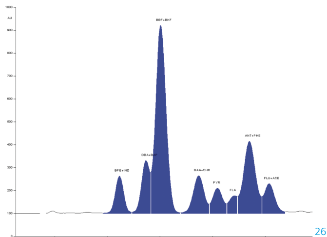
Fluorescence measurement of a standard mixture, exemplarily at 250 nm / >320 nm
