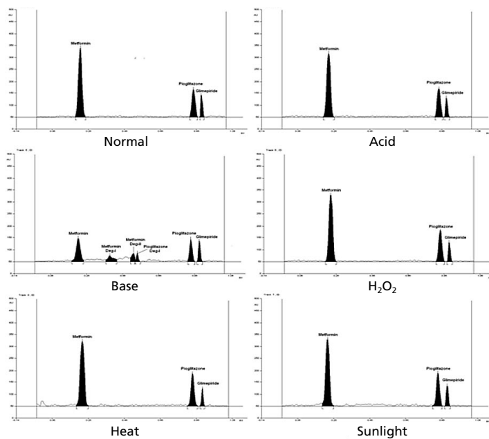
15 HPTLC densitograms of forced degradation study on pioglitazone, metformin and glimepiride. As can be seen, the stability was only affected in an alkaline medium.
