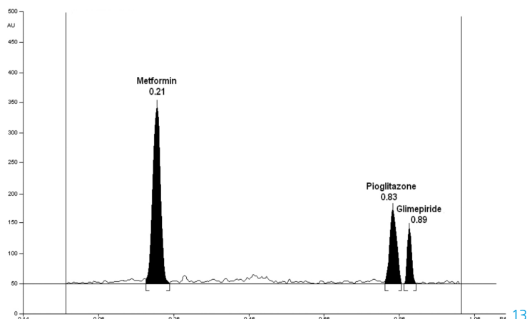
13 Separation of pioglitazone, metformine and glimepiride in marketed formulation
