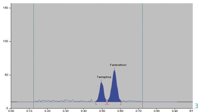
Densitogram, absorbance measurement at 290 nm
