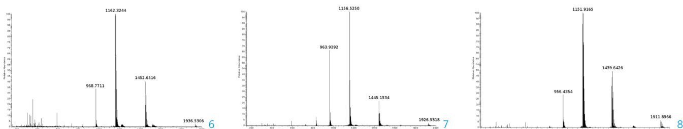
Reference spectra of human insulin (left), porcine insulin (mid) and bovine insulin (right)
