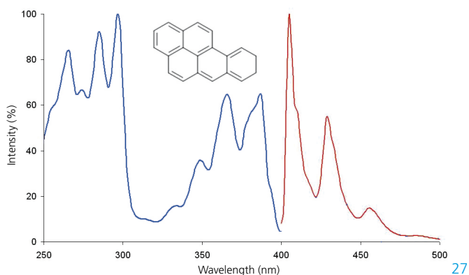
Fluorescence excitation spectrum (blue, \lambda_{ex} = 366 \text{ nm} ) and fluorescence emission spectrum (red, \lambda_{em} = 405 \text{ nm} ) of benzo[a]pyrene
