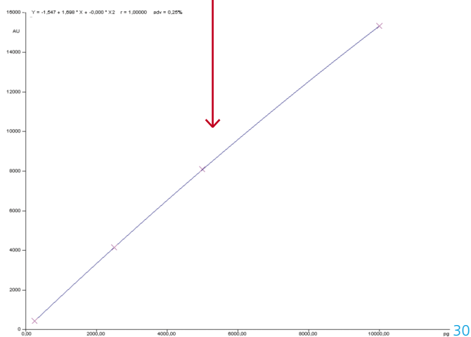
Calibration of benzo[a]pyrene (0.25–10 ng/zone), fluorescence measurement at 366 nm/>400 nm
