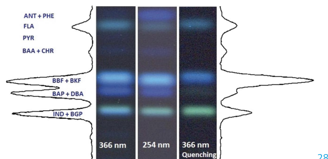
Plate images of a separated standard mixture (10 ng/zone) illuminated under different wavelengths and after fluorescence quenching by nitromethane; fluorescence scans at 366 nm / >400 nm
