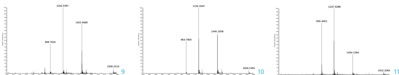
Human insulin (left), porcine insulin (mid) and bovine insulin (right) measured from the ProteoChrom® HPTLC silica gel 60 F 254s
