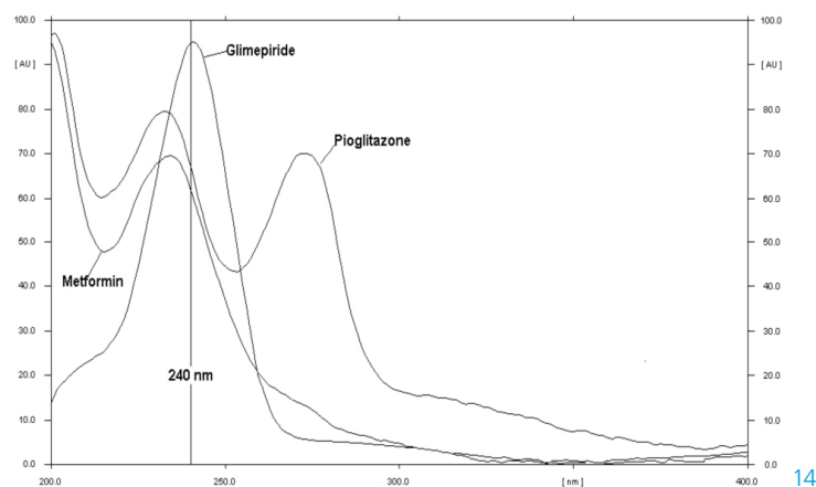
14 Spectra of Ziglil plus-2 tablet
