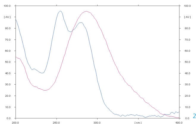
UV spectra 200–400 nm of temephos (blue) and fenitrothion (red)
